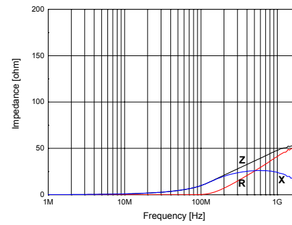
HH-1S1608-100J
