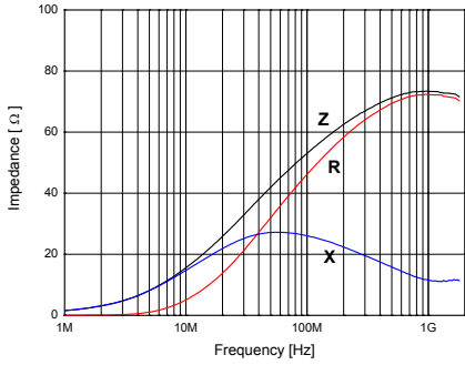
HH-1T3216-500J
