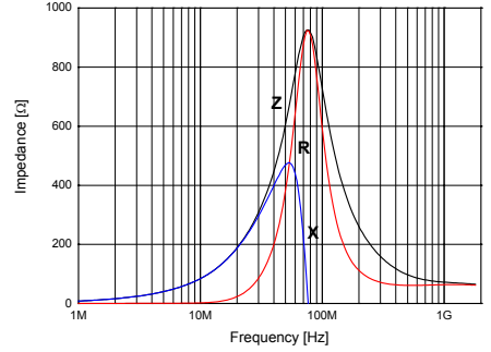
HH-1M4532-601J
