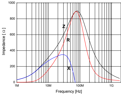
HH-1T3216-801J
