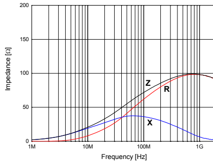
HH-1T3216-700J
