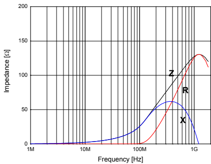
HH-1S1608-300J
