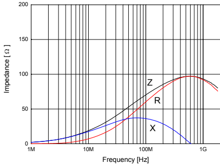
HB-1T1005-700J
