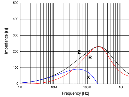
HH-1T3216-201J
