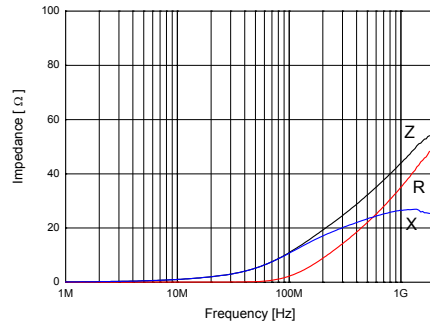
HB-1S1005-100J
