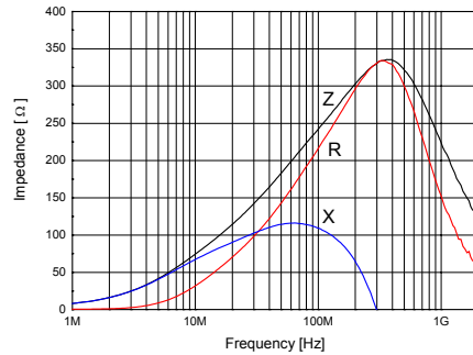
HB-1T1005-241J
