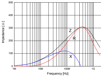
HB-1T1005-221J
