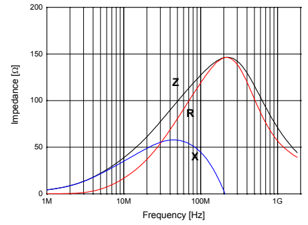
HH-1T3216-121J
