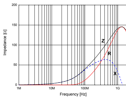
HH-1S1608-400J
