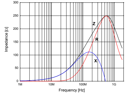
HH-1M1608-121J
