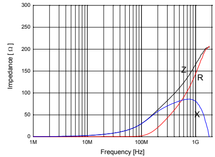
HB-1S1005-300J
