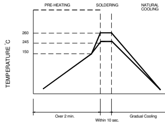
Figure 2. Wave Soldering
