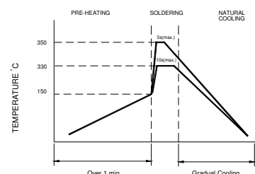
Figure 3. Hand Soldering
