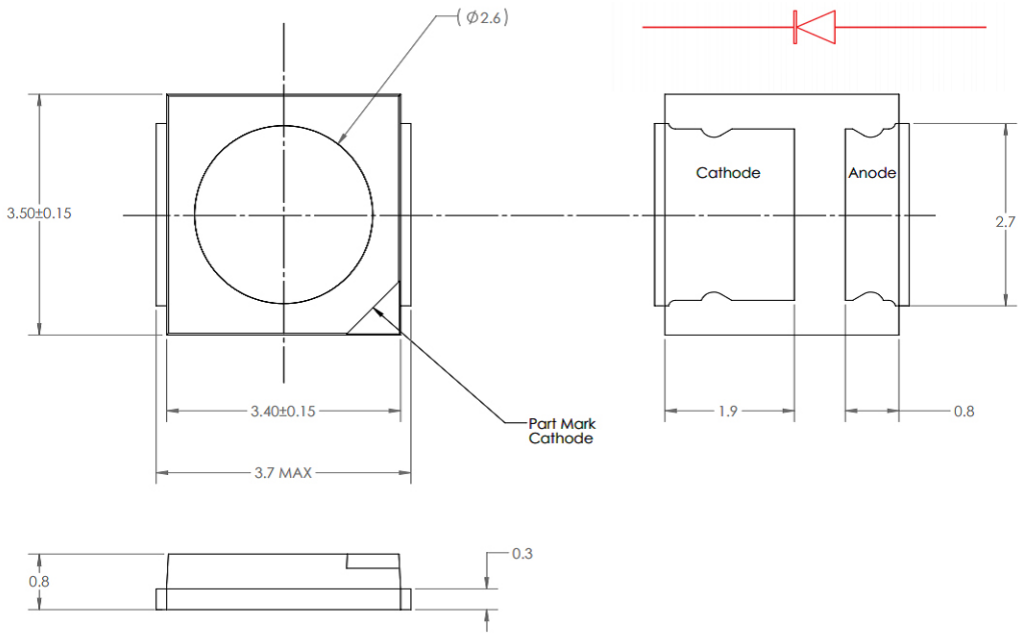
Figure 10: Mechanical dimensions for LUXEON 3535L Color Line of LEDs.
