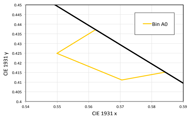
Figure 8: Color Bin Structure for LUXEON 3535L PC Amber for Table 9.
