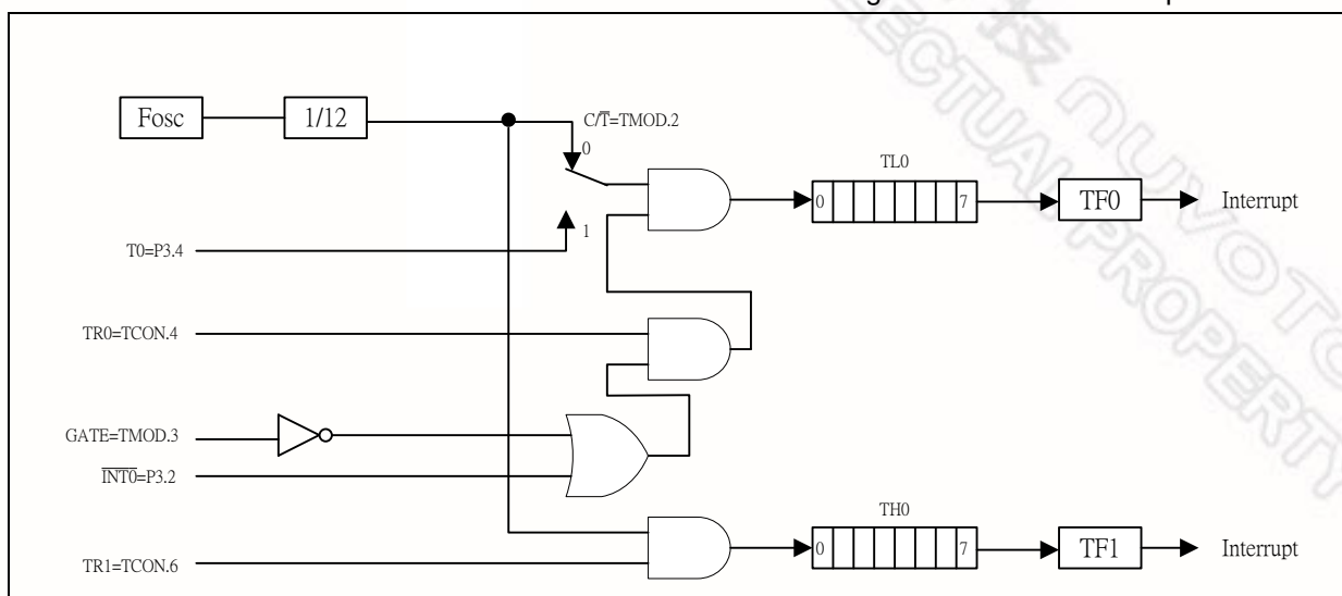
Figure 14-3 Timer/Counter Mode 3
